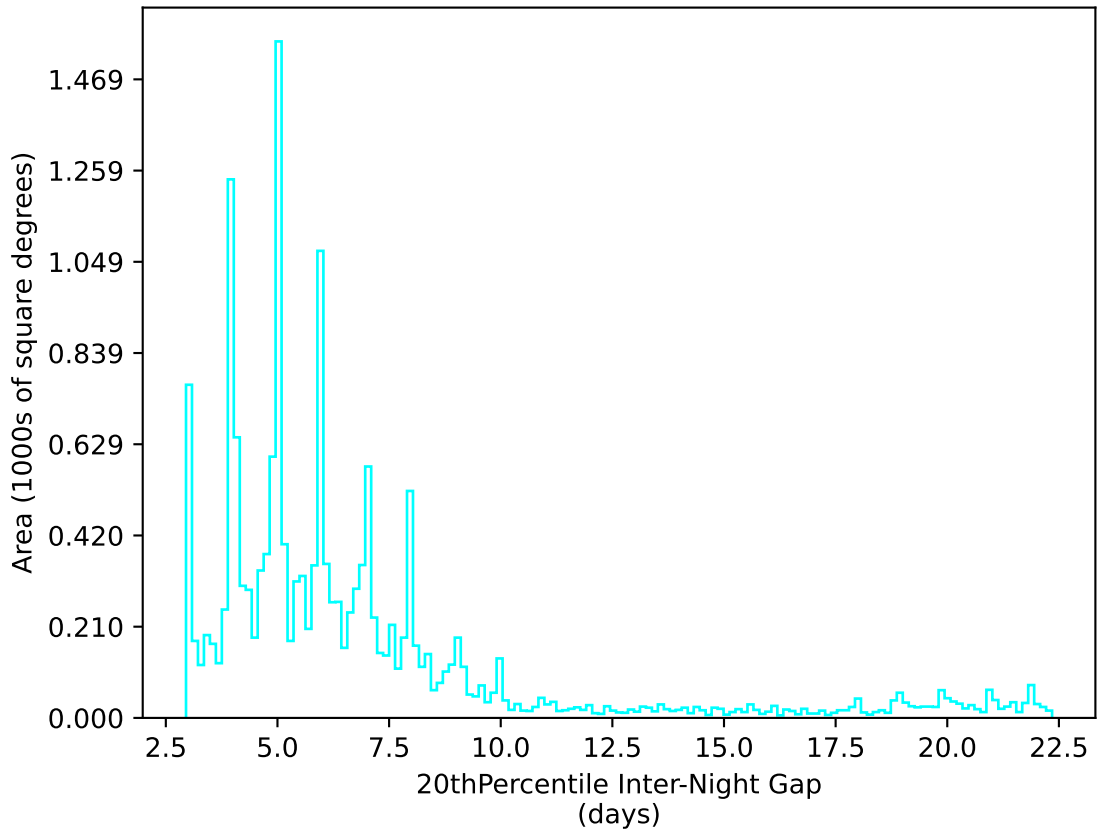
noroll_mjdp60_v3.4_10yrs WFD u band: 20thPercentile Inter-Night Gap
