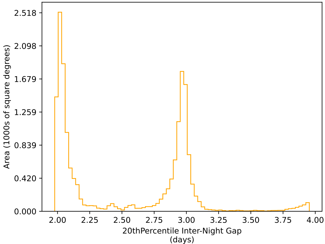
noroll_mjdp60_v3.4_10yrs WFD r band: 20thPercentile Inter-Night Gap
