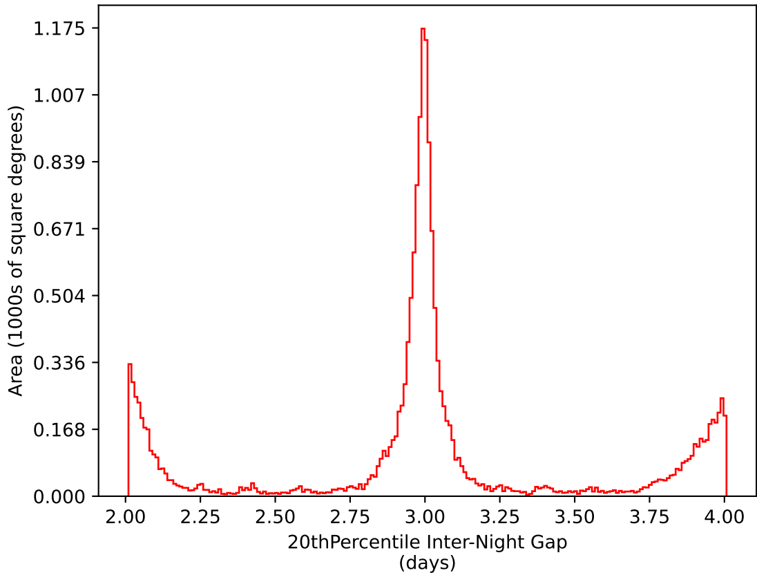
noroll_mjdp60_v3.4_10yrs WFD i band: 20thPercentile Inter-Night Gap
