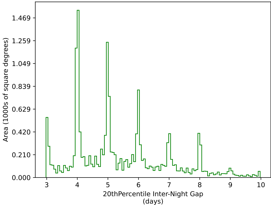
noroll_mjdp60_v3.4_10yrs WFD g band: 20thPercentile Inter-Night Gap
