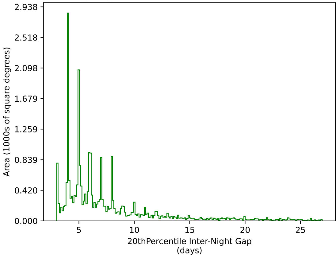
noroll_mjdp60_v3.4_10yrs All sky g band: 20thPercentile Inter-Night Gap
