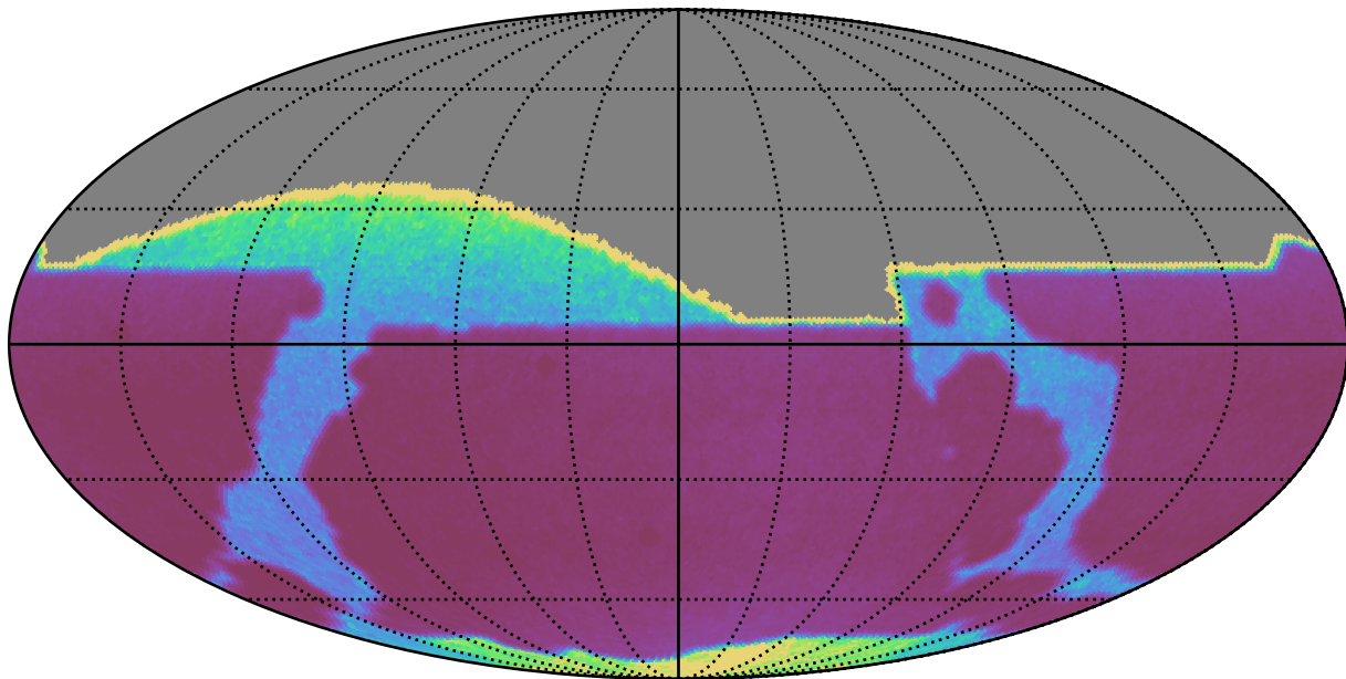
noroll_mjdp60_v3.4_10yrs : properMotion
