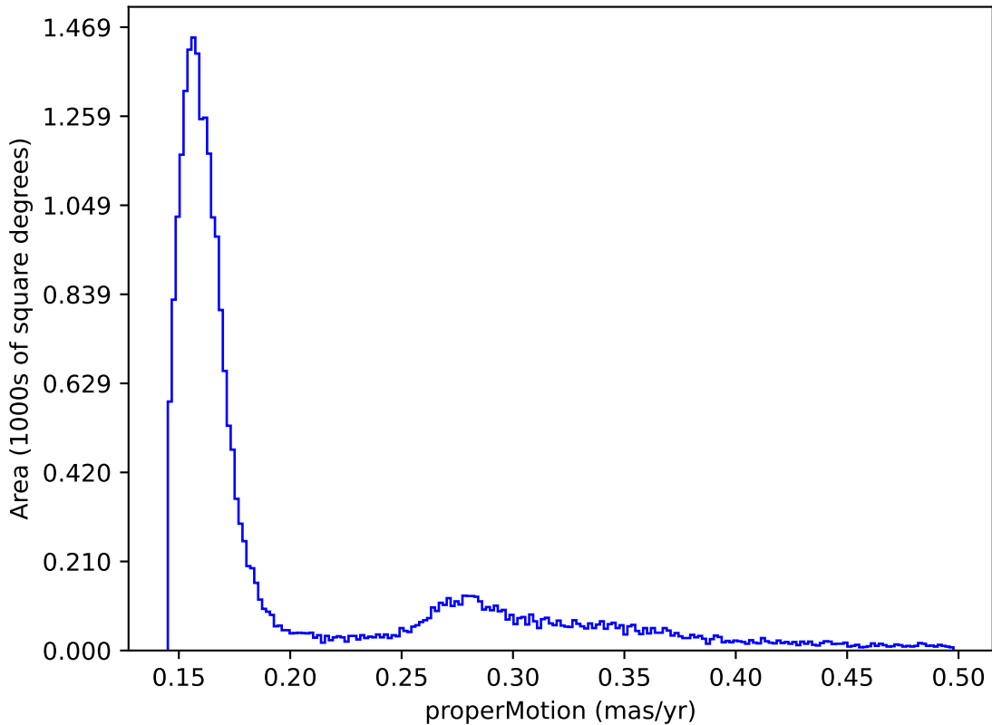
noroll_mjdp60_v3.4_10yrs : properMotion
