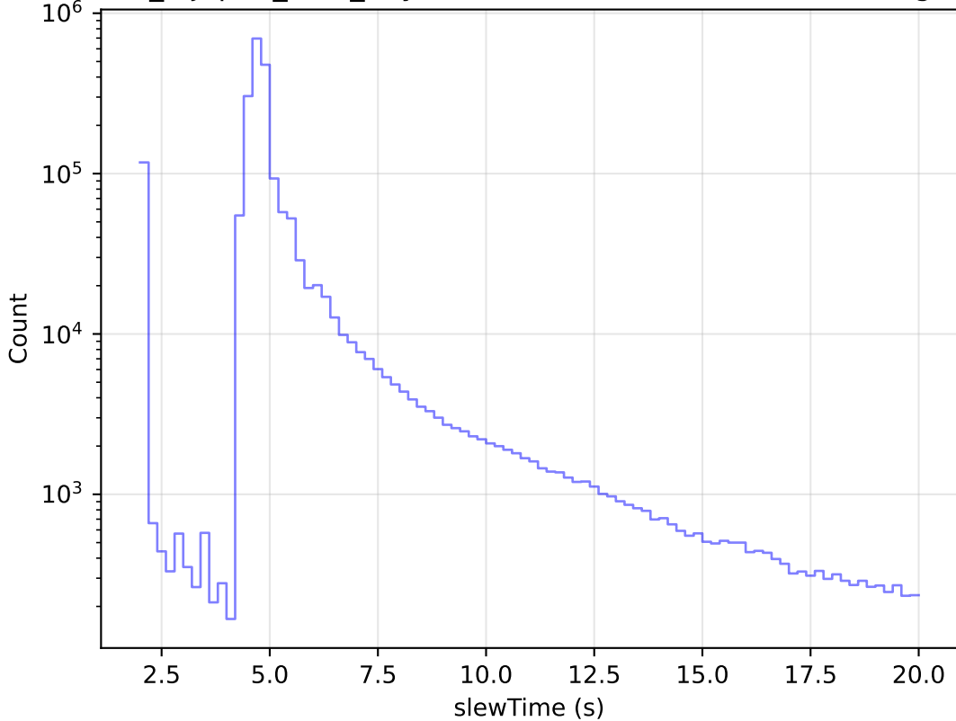
noroll_mjdp60_v3.4_10yrs All visits: Zoom Slew Time Histogram
