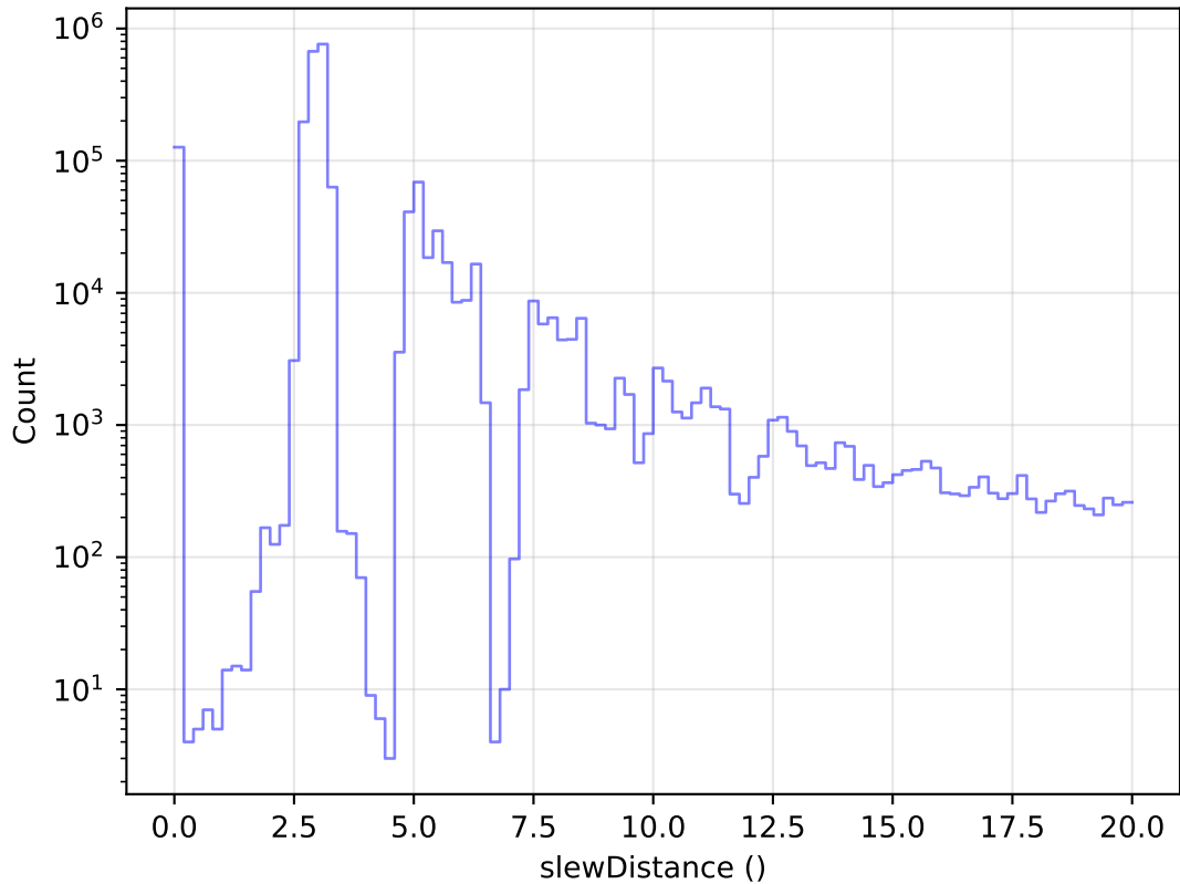
noroll_mjdp60_v3.4_10yrs All visits: Zoom Slew Distance Histogram
