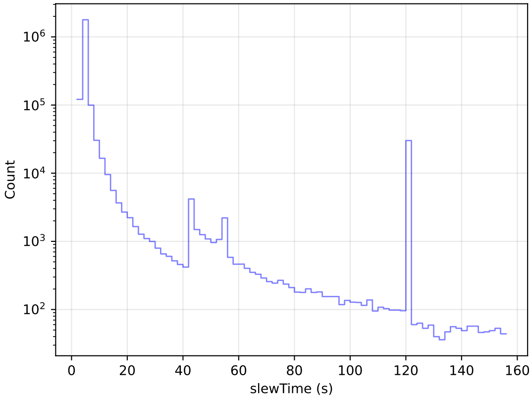
noroll_mjdp60_v3.4_10yrs All visits: Slew Time Histogram
