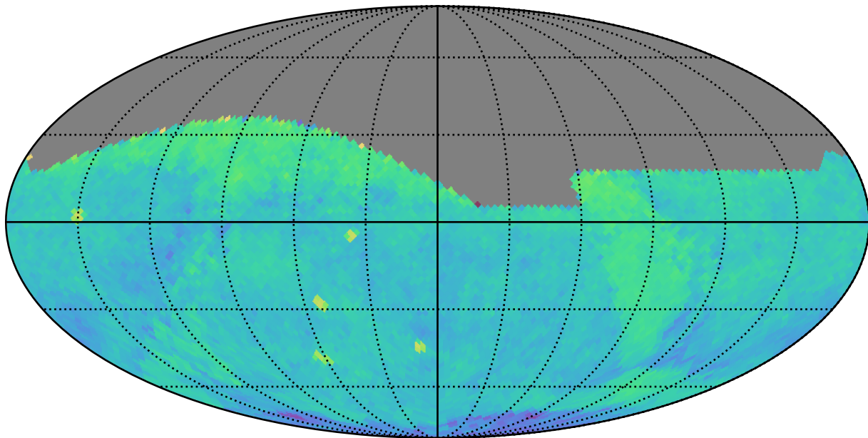
noroll_mjdp60_v3.4_10yrs (g or r or i): PairFraction
