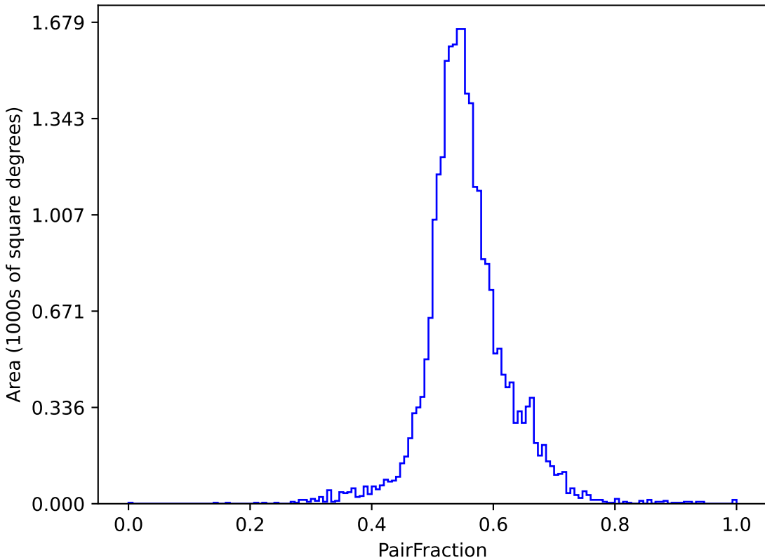
noroll_mjdp60_v3.4_10yrs (g or r or i): PairFraction
