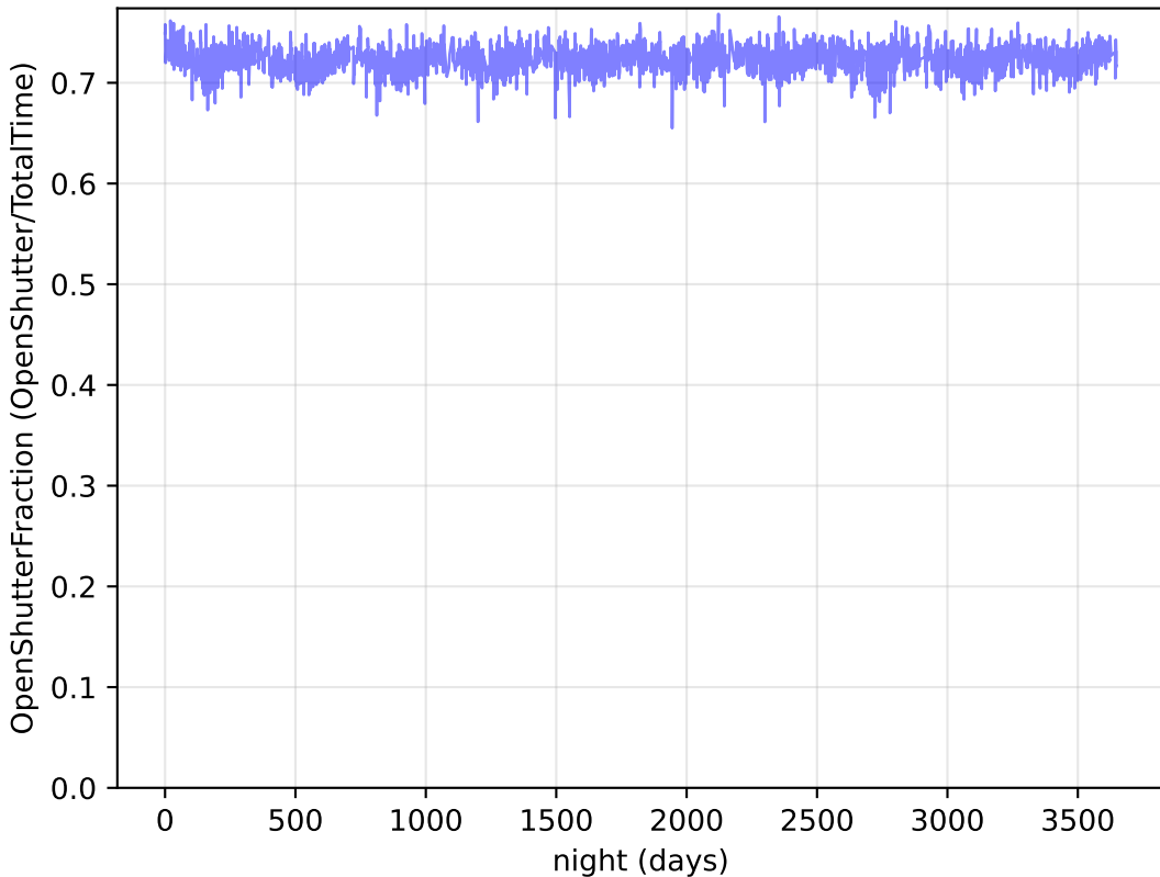
noroll_mjdp60_v3.4_10yrs : OpenShutterFraction
