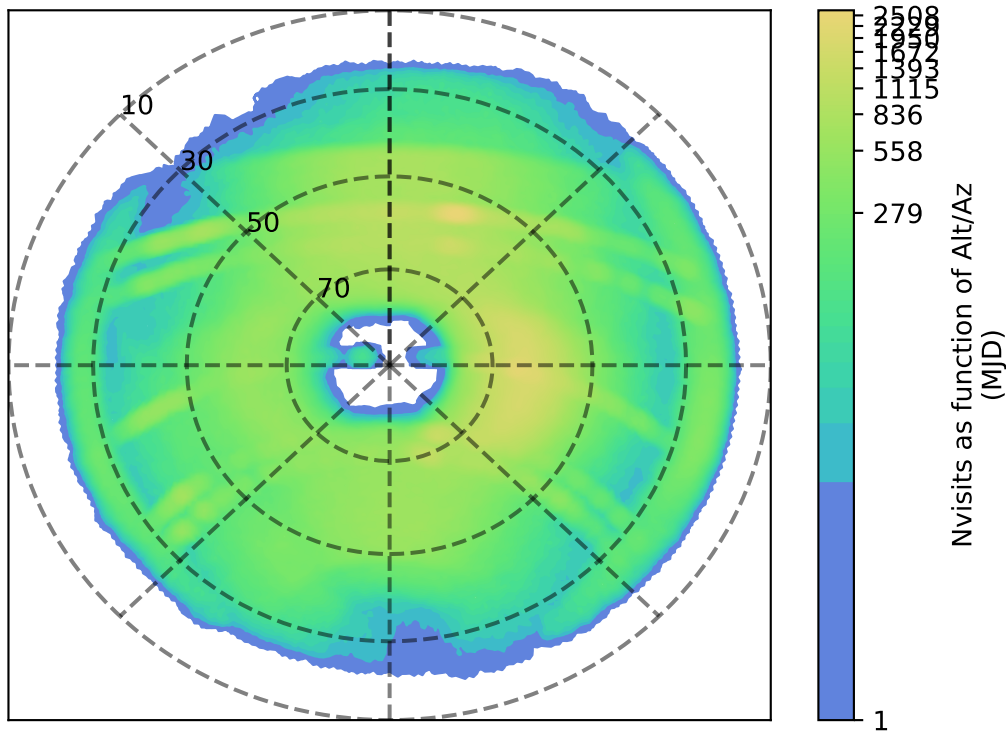
noroll_mjdp60_v3.4_10yrs z: Nvisits as function of Alt/Az
