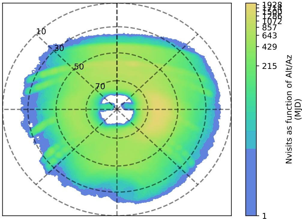
noroll_mjdp60_v3.4_10yrs y: Nvisits as function of Alt/Az
