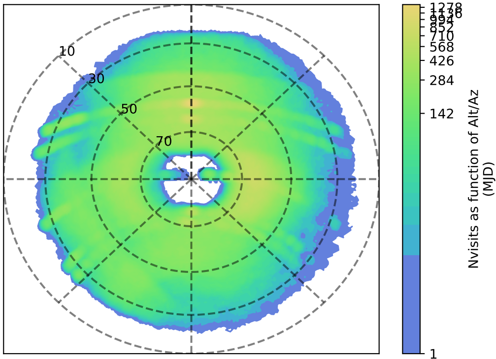
noroll_mjdp60_v3.4_10yrs g: Nvisits as function of Alt/Az
