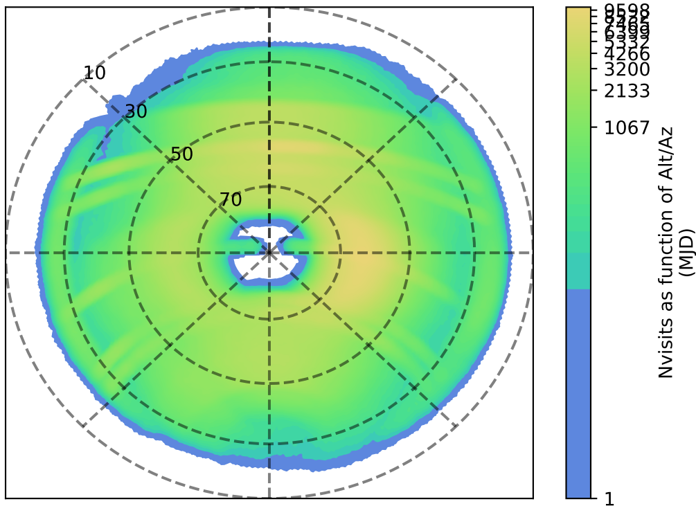
noroll_mjdp60_v3.4_10yrs : Nvisits as function of Alt/Az
