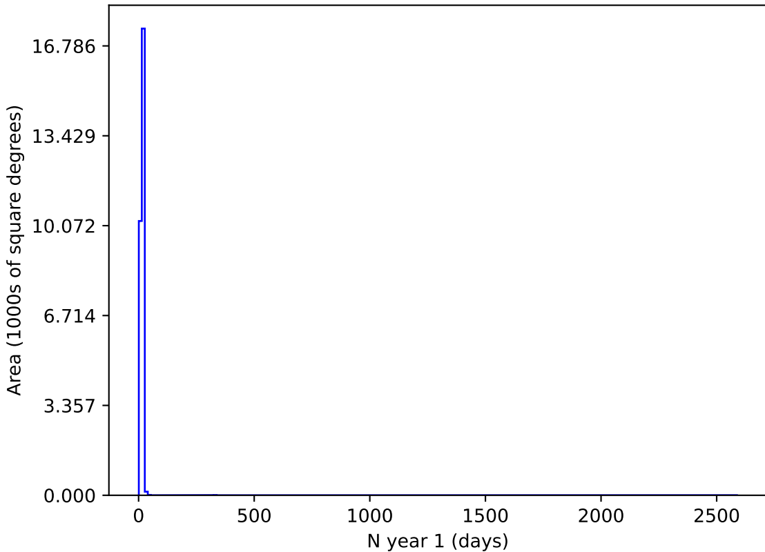
noroll_mjdp60_v3.4_10yrs z and night < 365: N year 1
