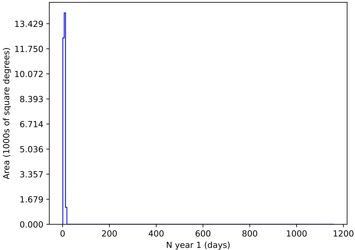
noroll_mjdp60_v3.4_10yrs g and night < 365: N year 1
