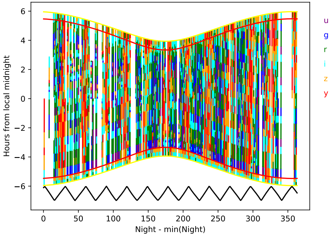
noroll_mjdp60_v3.4_10yrs year 9-10: Hourglass
