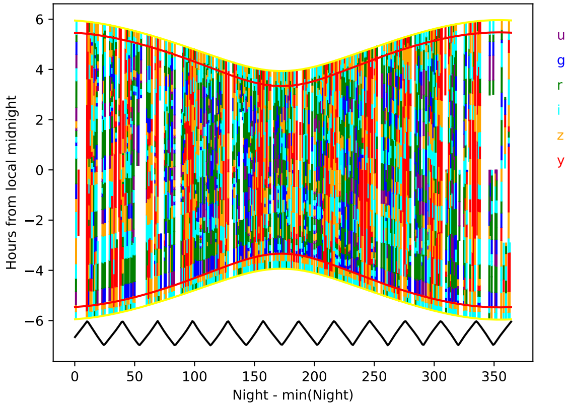
noroll_mjdp60_v3.4_10yrs year 8-9: Hourglass
