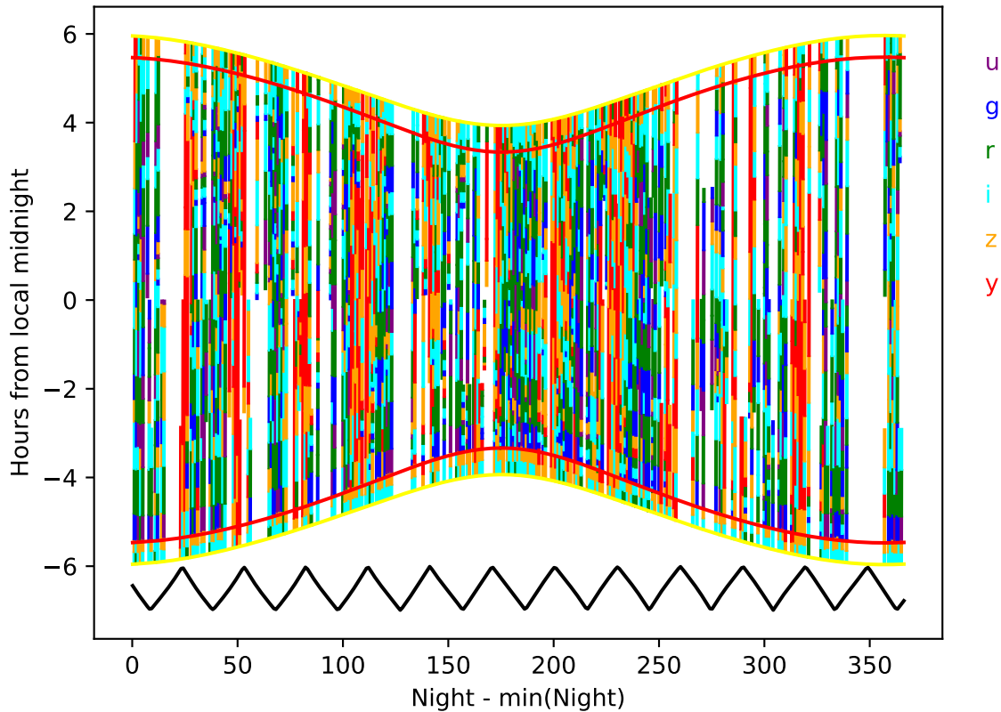
noroll_mjdp60_v3.4_10yrs year 7-8: Hourglass
