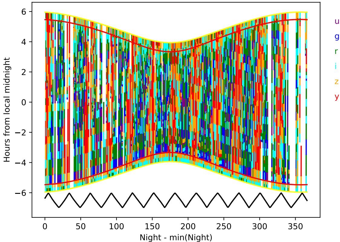
noroll_mjdp60_v3.4_10yrs year 6-7: Hourglass
