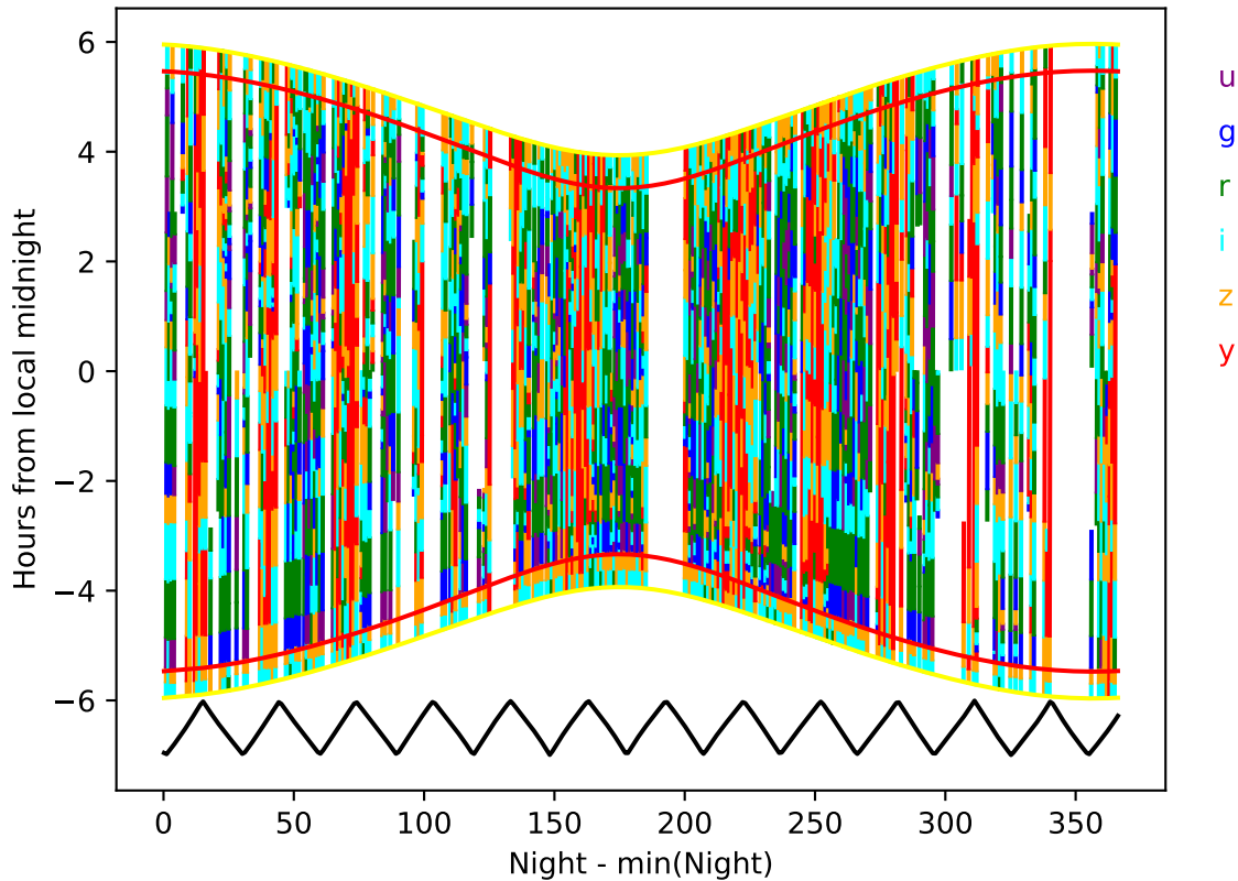
noroll_mjdp60_v3.4_10yrs year 5-6: Hourglass
