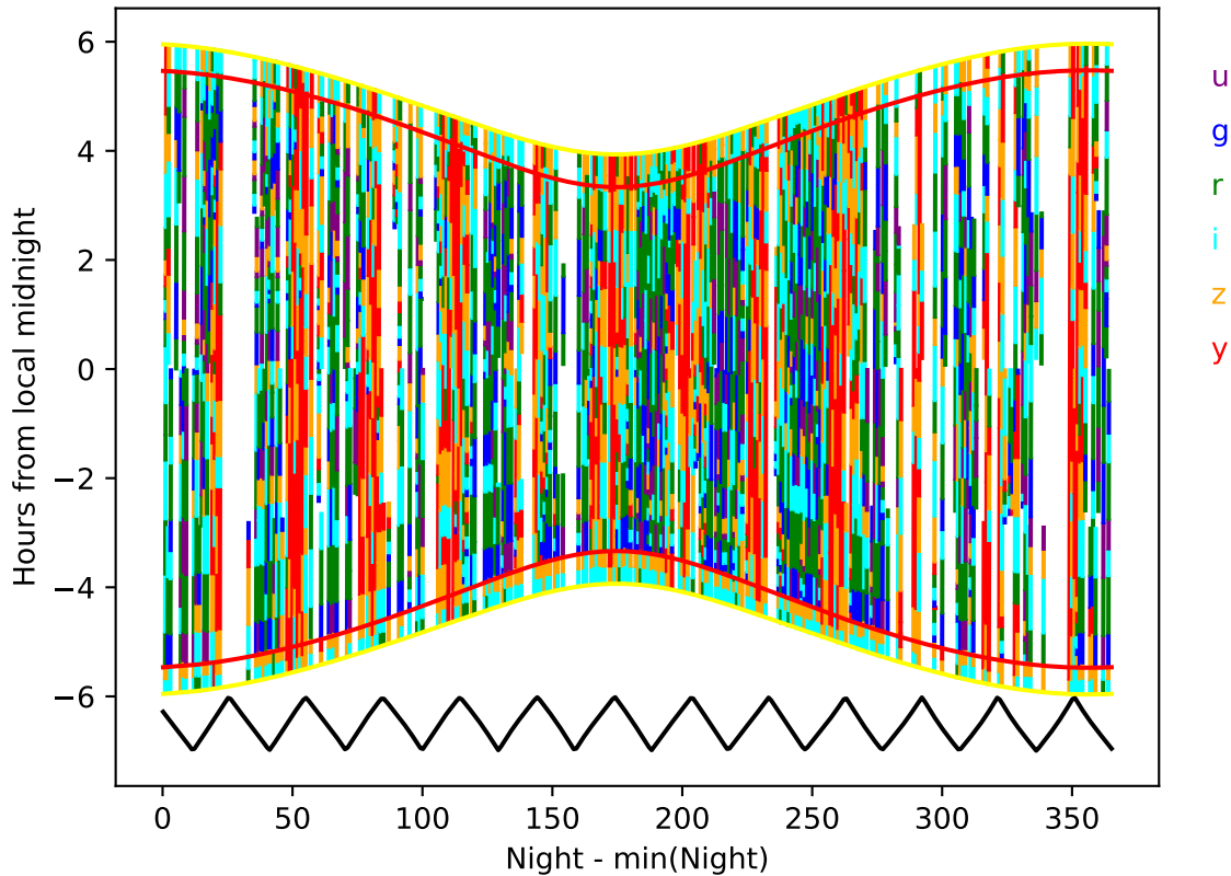
noroll_mjdp60_v3.4_10yrs year 4-5: Hourglass
