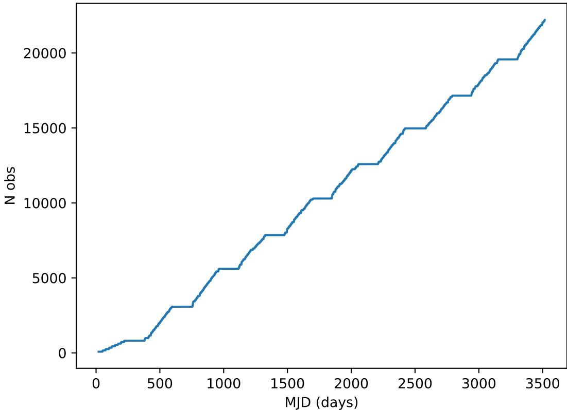
noroll_mjdp60_v3.4_10yrs note like DD:XMM_LSS%: Cumulative
