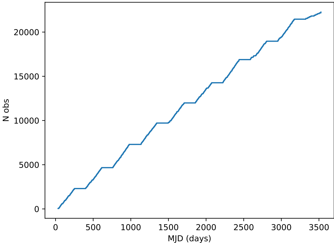
noroll_mjdp60_v3.4_10yrs note like DD:ECDFS%: Cumulative
