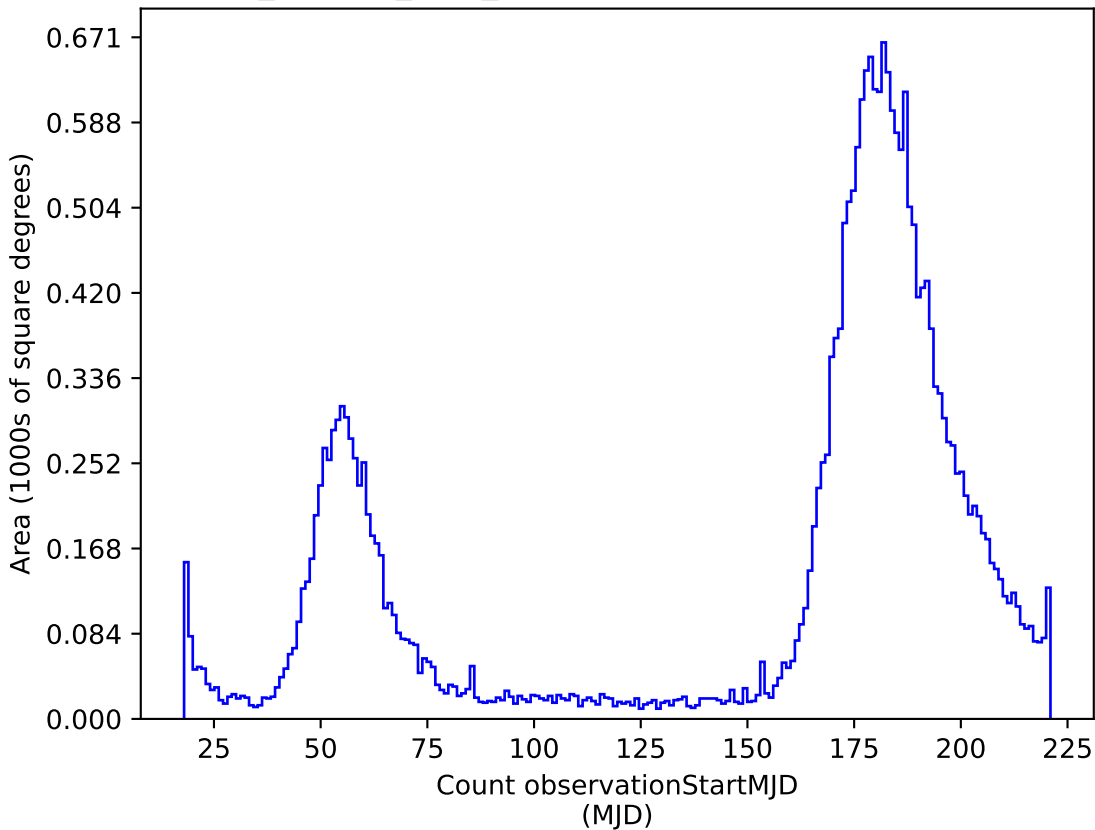
noroll_mjdp60_v3.4_10yrs r: Count observationStartMJD
