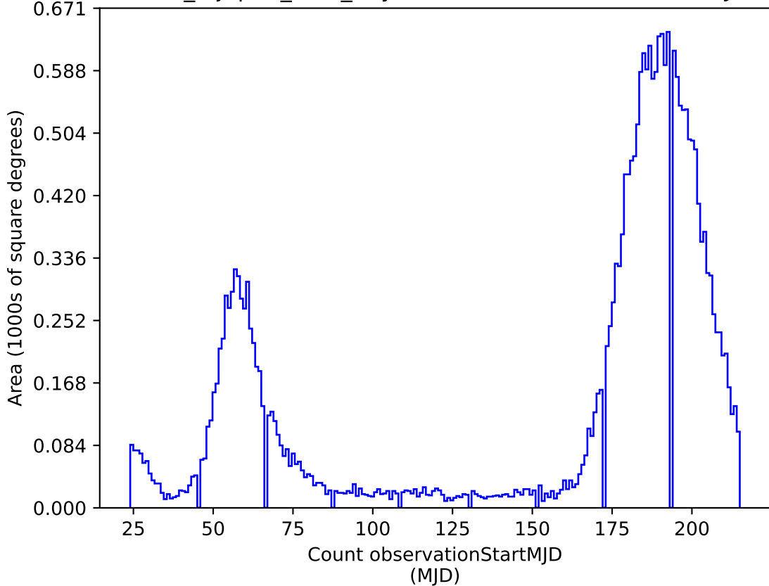
noroll_mjdp60_v3.4_10yrs i: Count observationStartMJD
