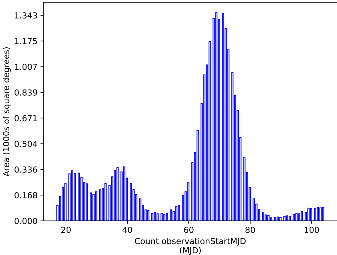
noroll_mjdp60_v3.4_10yrs g: Count observationStartMJD
