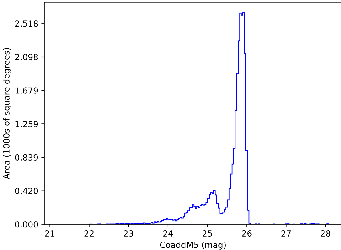
noroll_mjdp60_v3.4_10yrs z: CoaddM5
