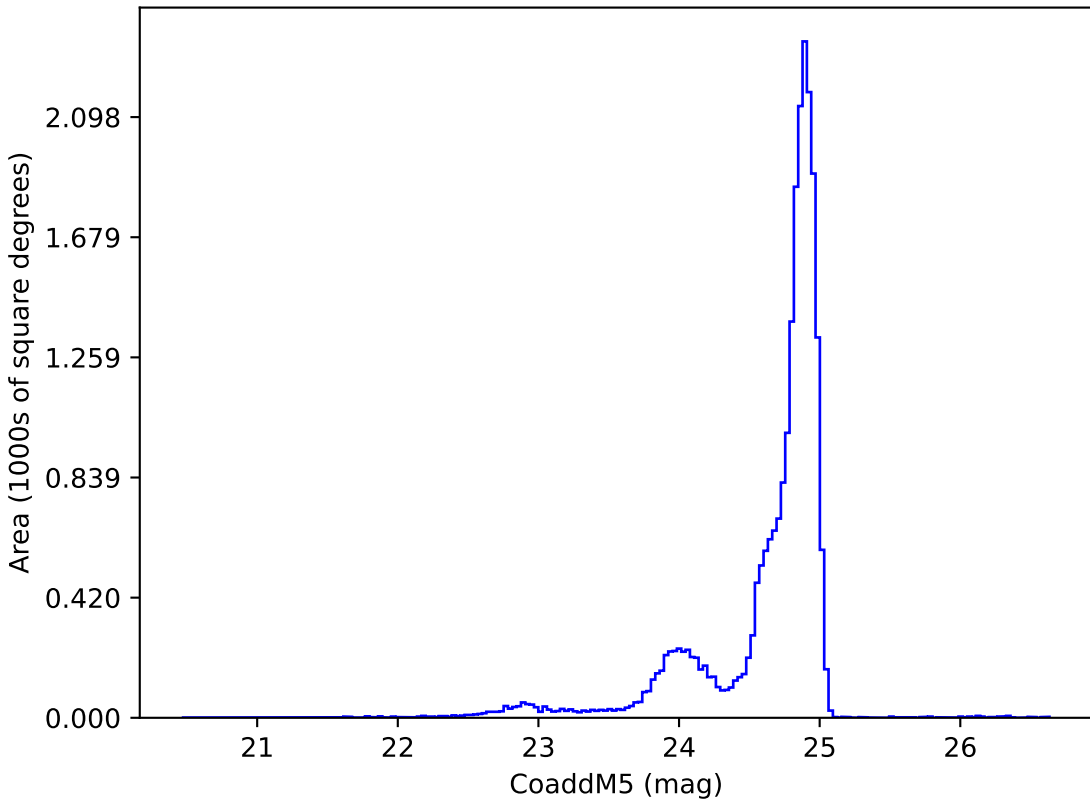
noroll_mjdp60_v3.4_10yrs y: CoaddM5
