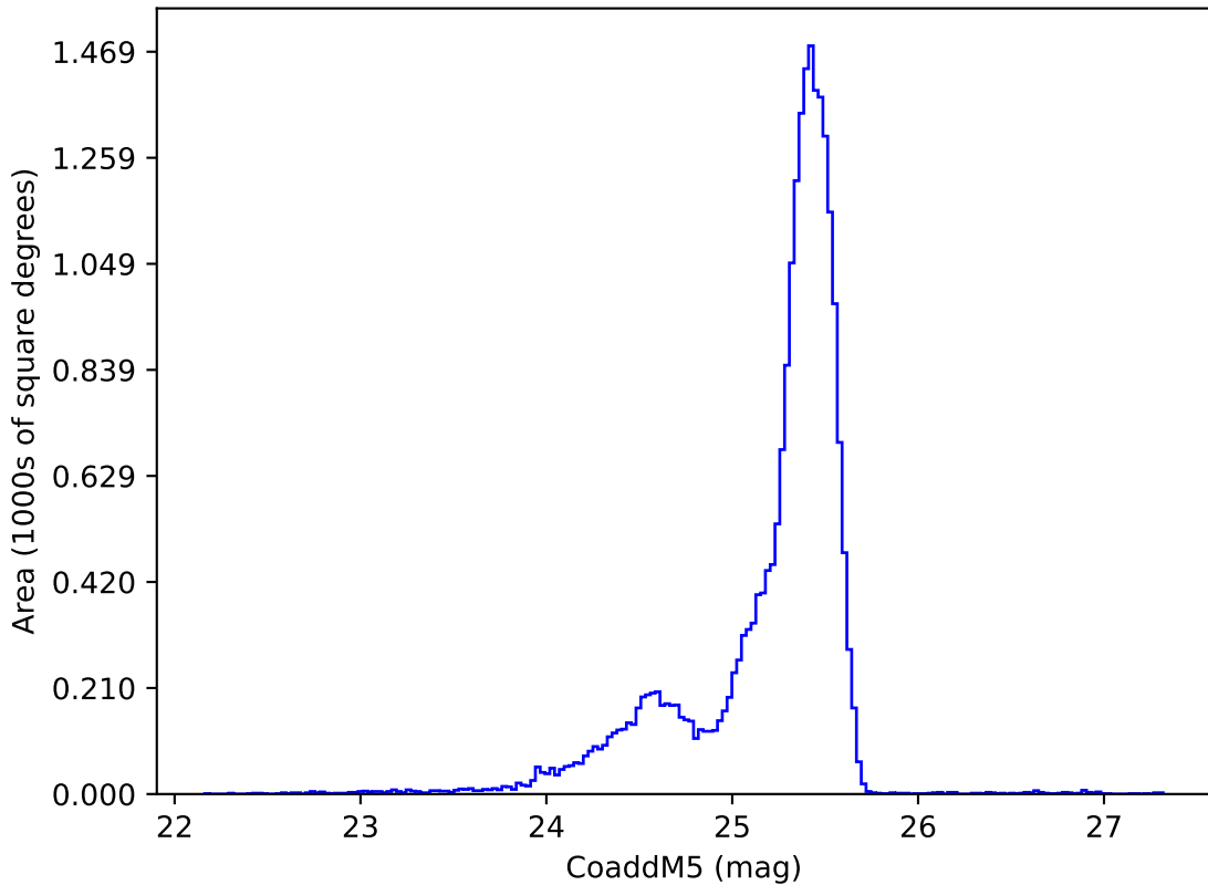
noroll_mjdp60_v3.4_10yrs u: CoaddM5
