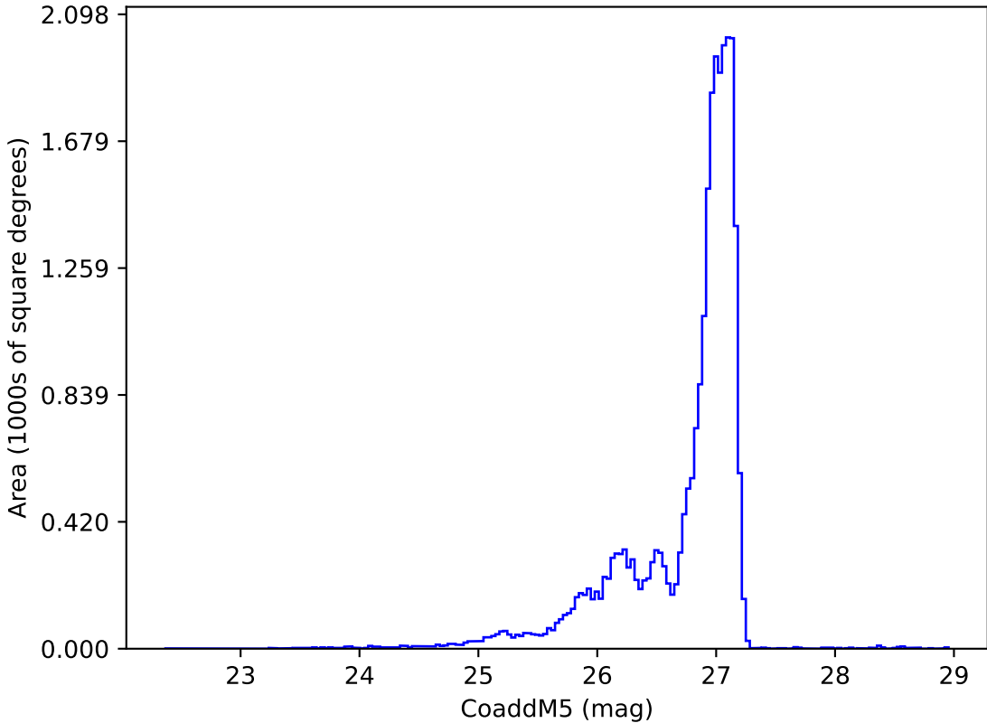
noroll_mjdp60_v3.4_10yrs r: CoaddM5
