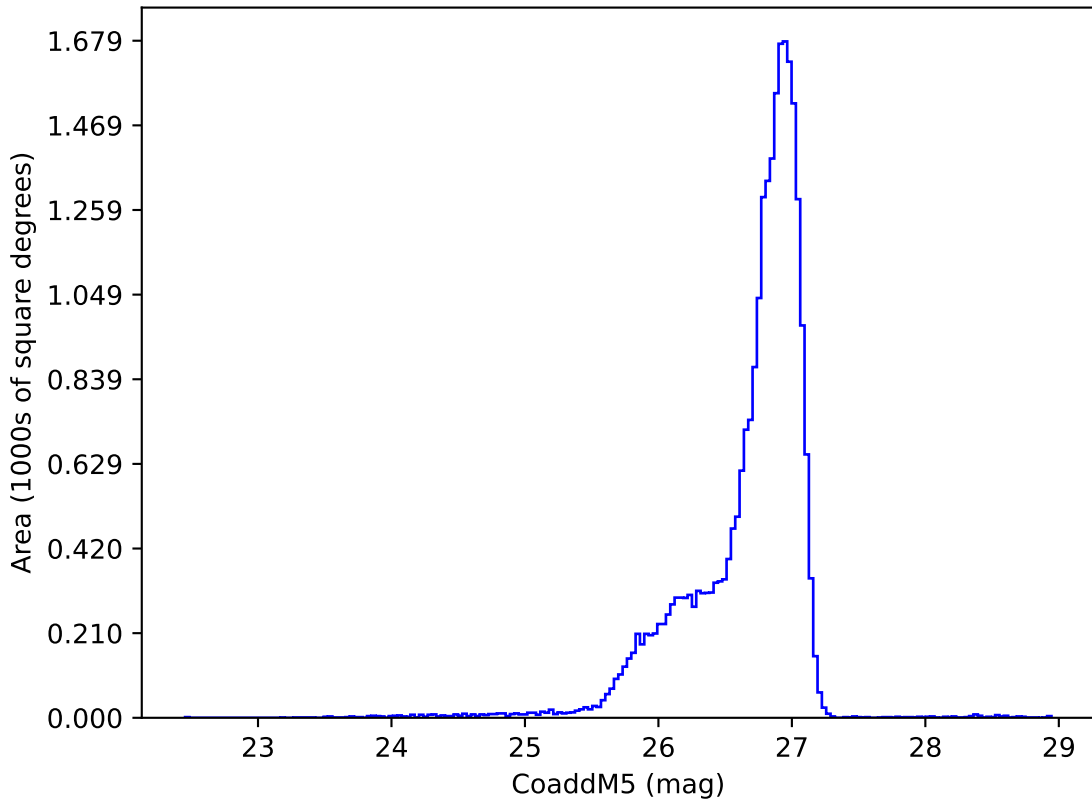
noroll_mjdp60_v3.4_10yrs g: CoaddM5
