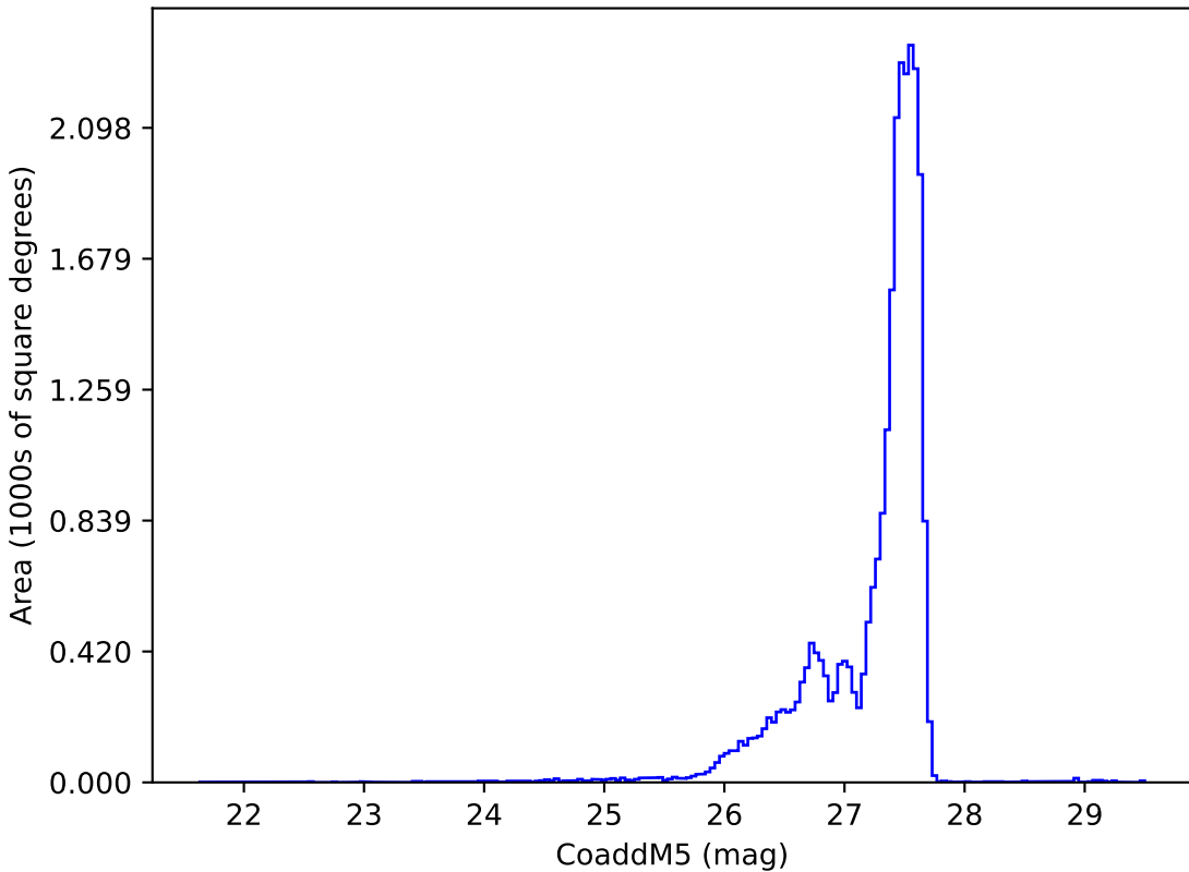
noroll_mjdp60_v3.4_10yrs : CoaddM5
