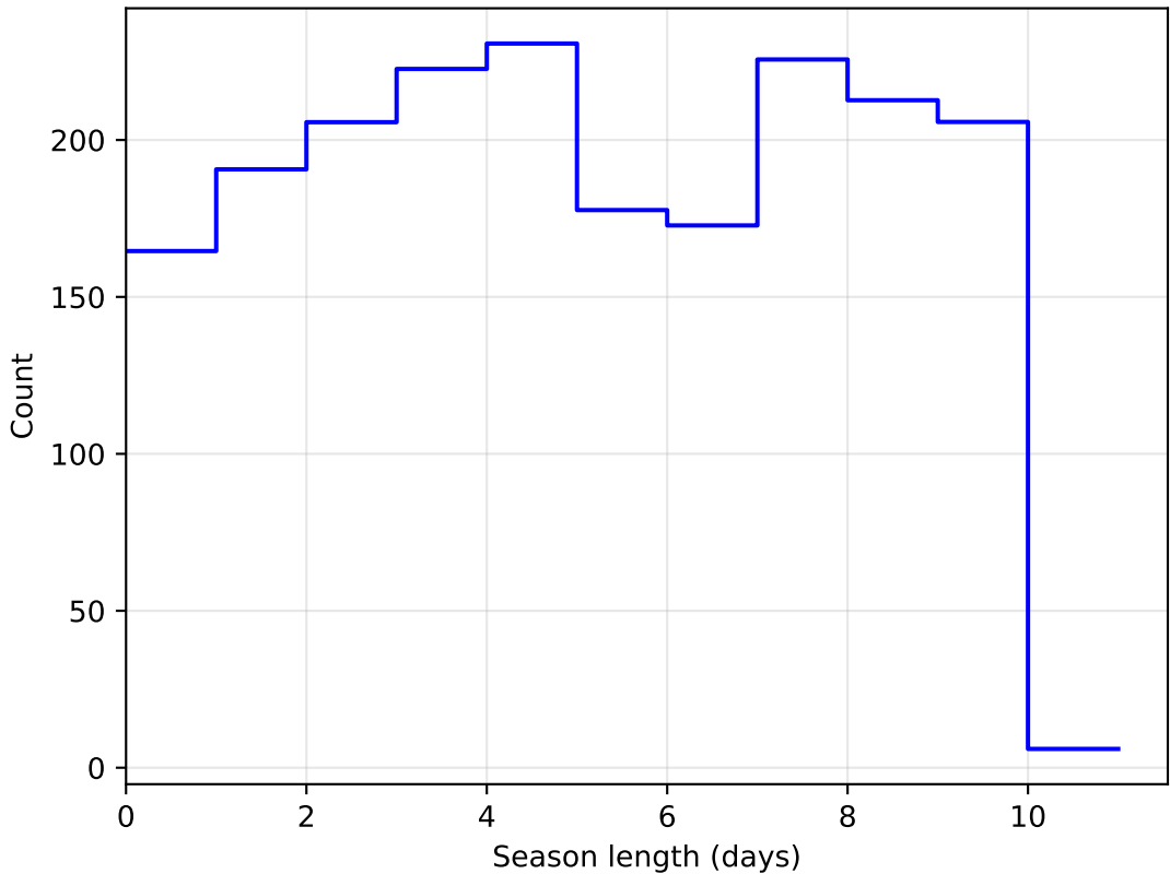
noroll_mjdp60_v3.4_10yrs DD:WFD all bands: SeasonLength
