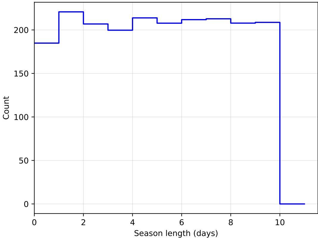
noroll_mjdp60_v3.4_10yrs DD:ELAISS1 all bands: SeasonLength
