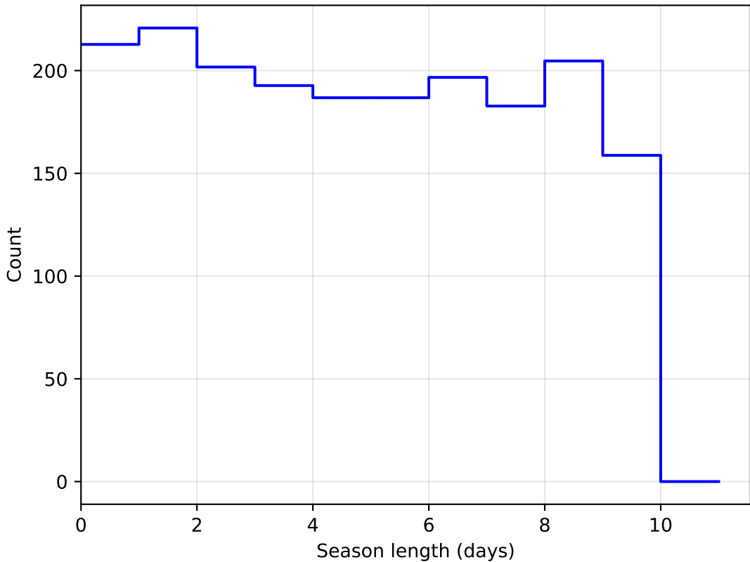
noroll_mjdp60_v3.4_10yrs DD: COSMOS all bands: SeasonLength
