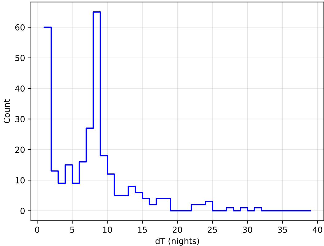
noroll_mjdp60_v3.4_10yrs all bands: DD:XMM_LSS Delta Nights Histogram
