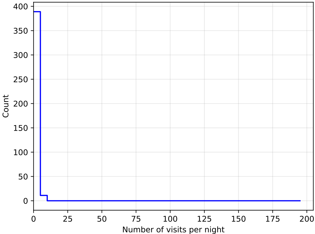
noroll_mjdp60_v3.4_10yrs all bands: DD:WFD NVisitsPerNight
