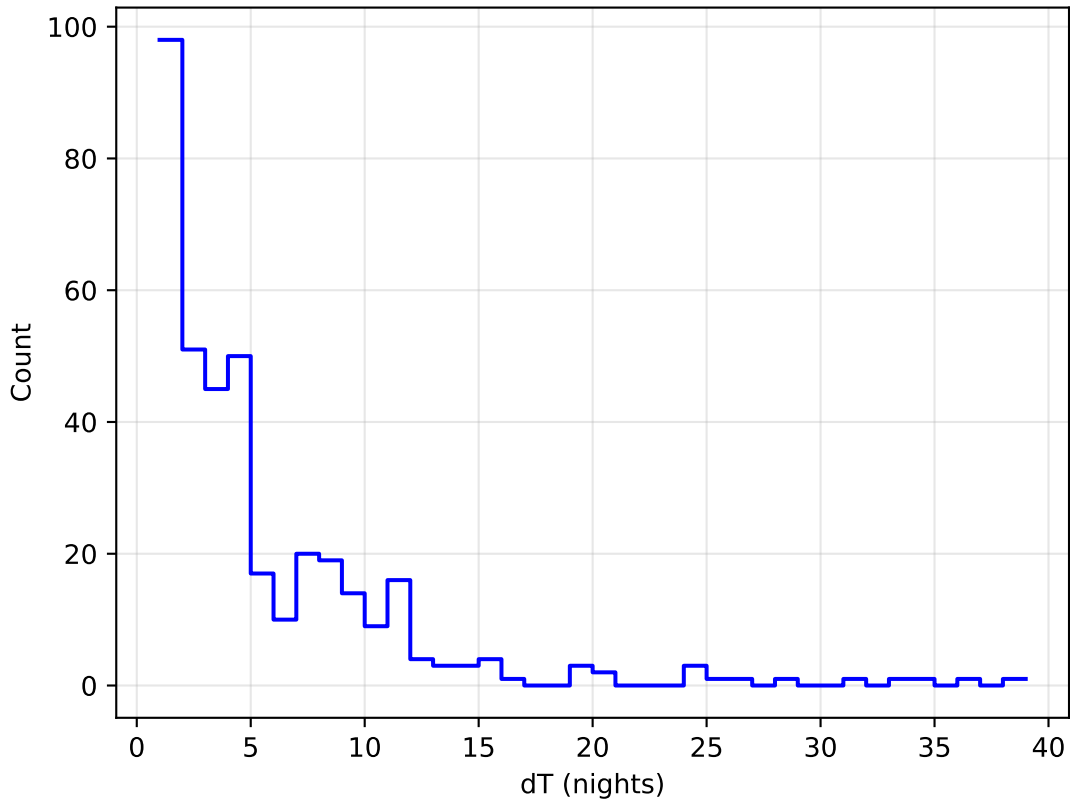
noroll_mjdp60_v3.4_10yrs all bands: DD:WFD Delta Nights Histogram
