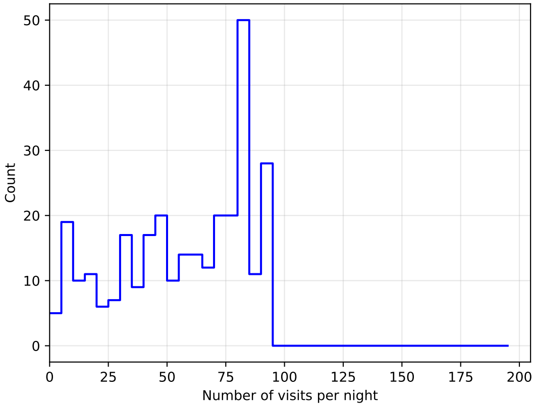
noroll_mjdp60_v3.4_10yrs all bands: DD:EDFS NVisitsPerNight
