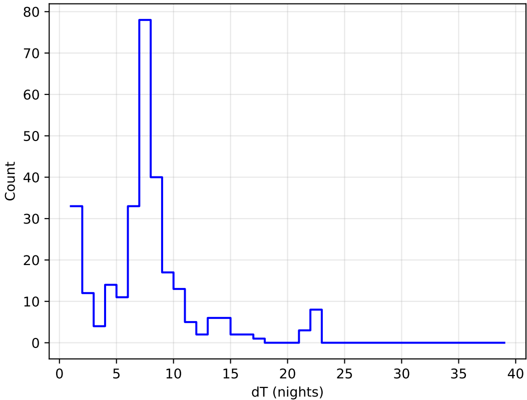
noroll_mjdp60_v3.4_10yrs all bands: DD:EDFS Delta Nights Histogram
