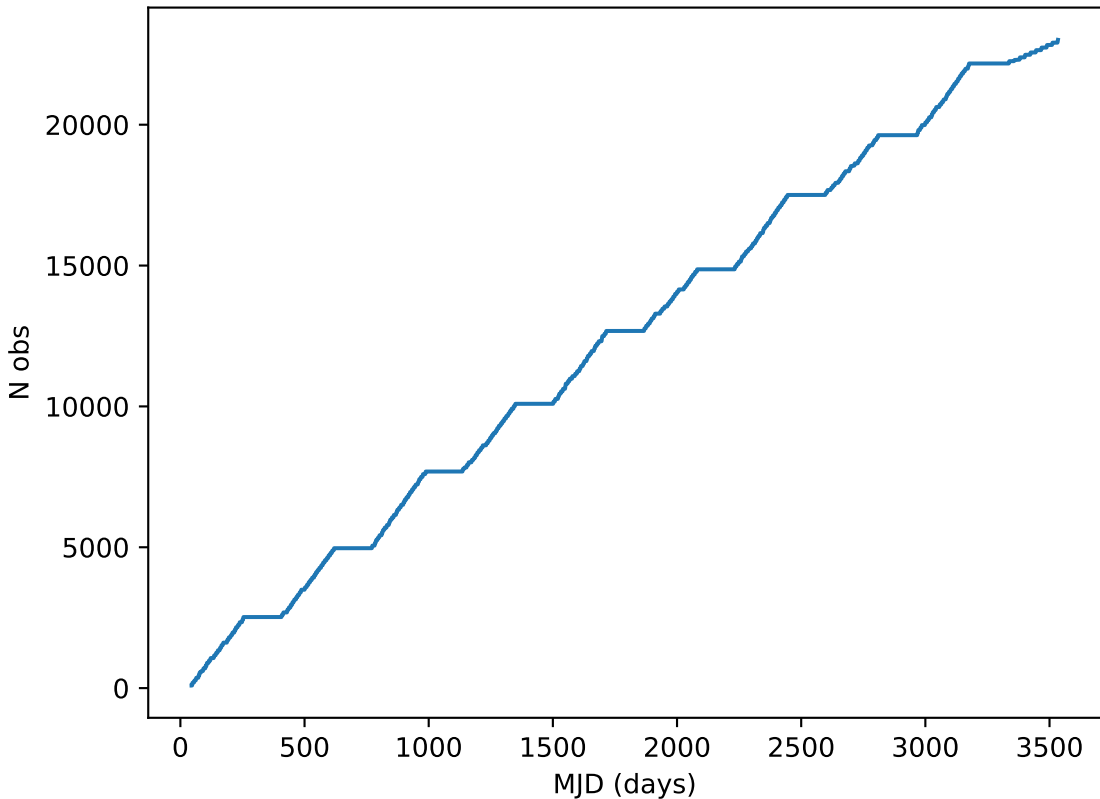
noroll_mjdp60_v3.4_10yrs all bands: DD:EDFS Cumulative NVisits
