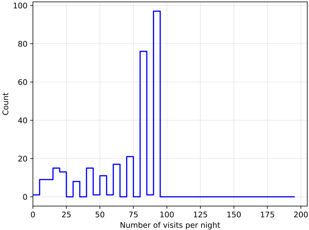
noroll_mjdp60_v3.4_10yrs all bands: DD:ECDFS NVisitsPerNight
