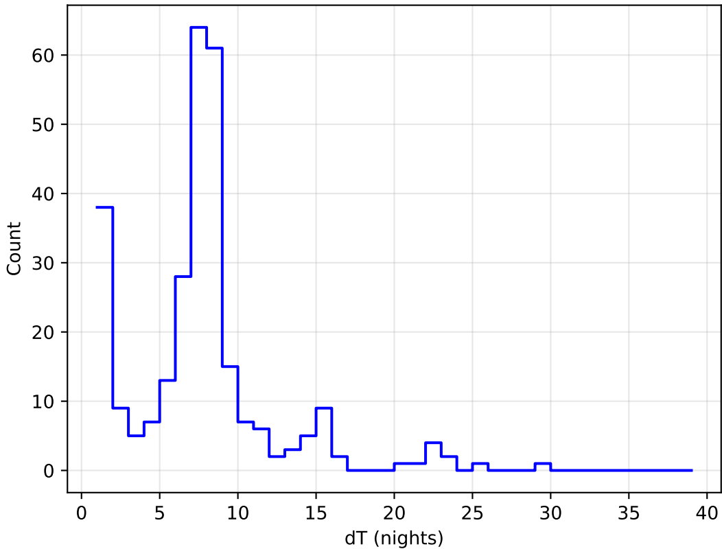
noroll_mjdp60_v3.4_10yrs all bands: DD:ECDFS Delta Nights Histogram
