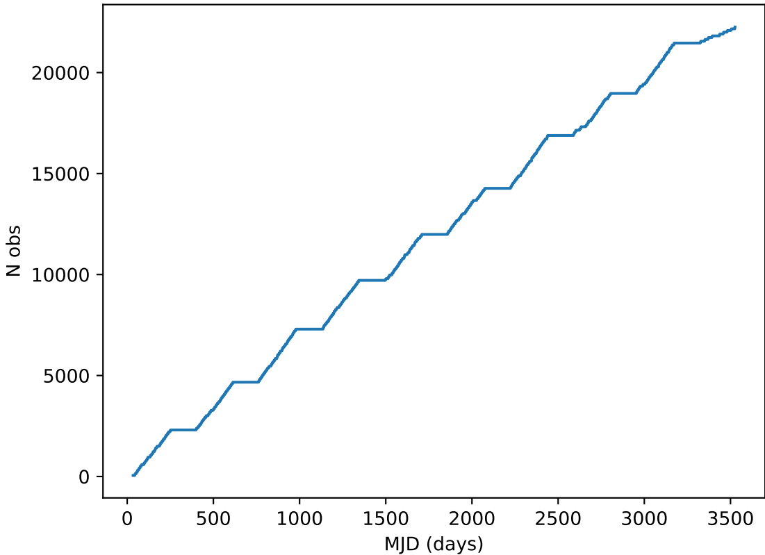
noroll_mjdp60_v3.4_10yrs all bands: DD:ECDFS Cumulative NVisits
