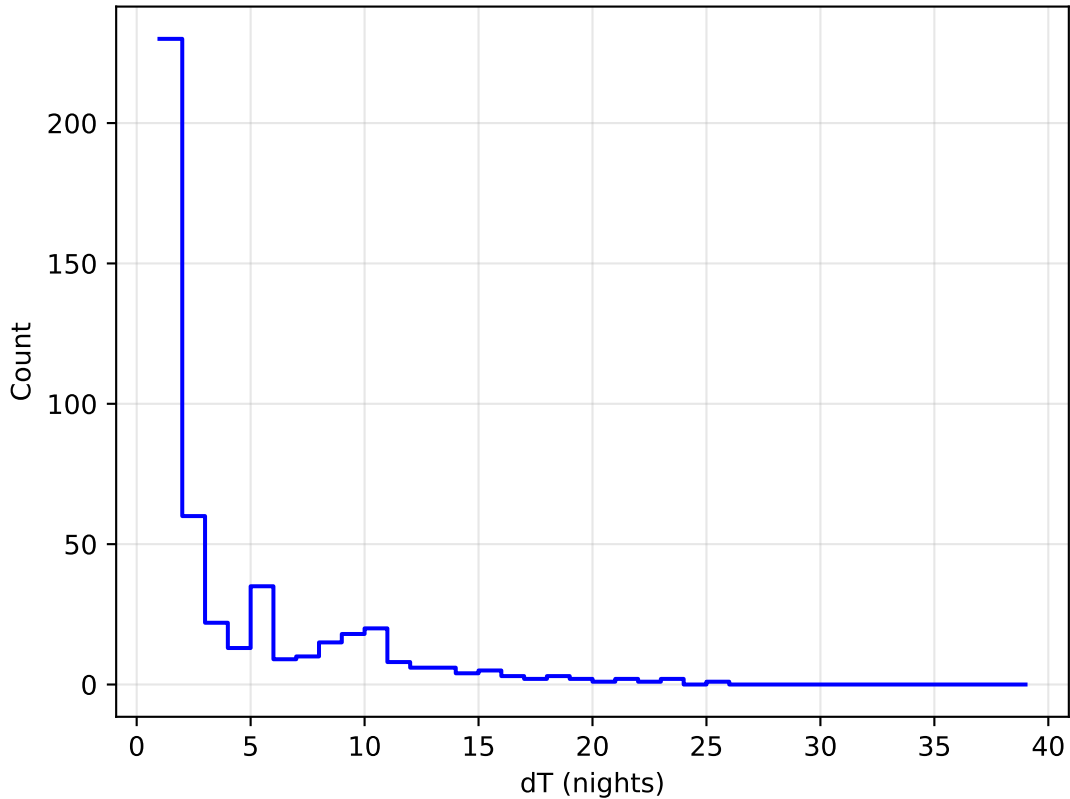
noroll_mjdp60_v3.4_10yrs all bands: DD: COSMOS Delta Nights Histogram
