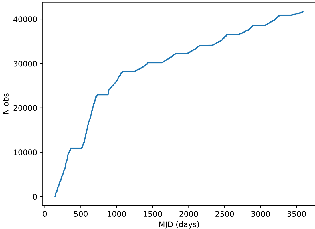
noroll_mjdp60_v3.4_10yrs all bands: DD:COSMOS Cumulative NVisits
